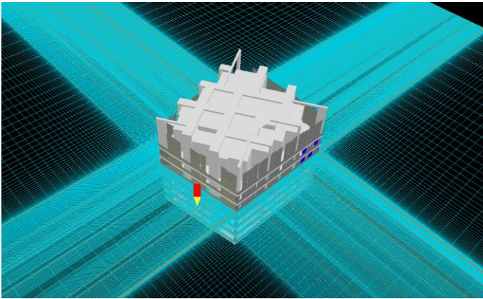
Fig. 5. PHOENICS model with grid.
