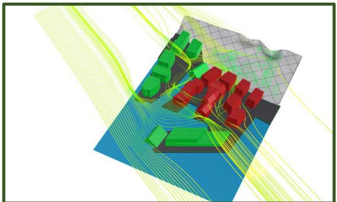
Velocity Stream Lines Shaded
