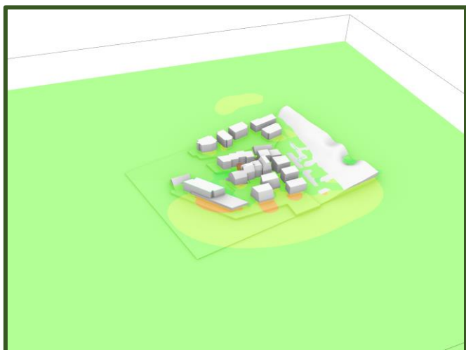
Pressure Cut Plane Contours
