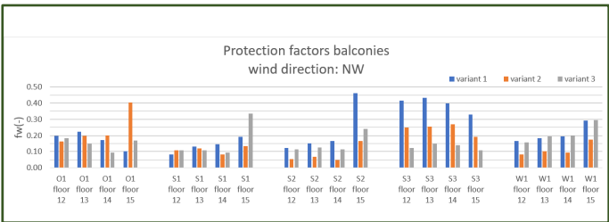
Fig. 6. Comparison of protection factors for different balconies on different floors for the 3 variants.
