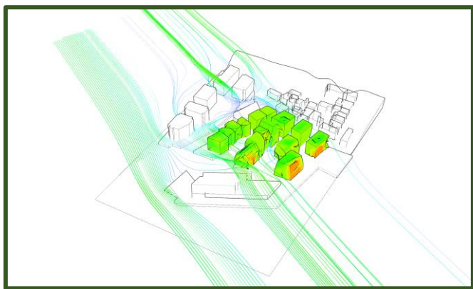
Velocity Stream Lines and Surface Contours
