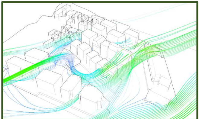
Velocity Stream Lines
