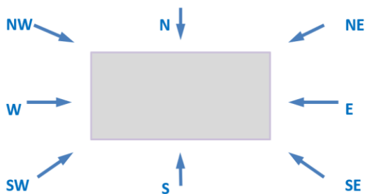
Fig. 2. Wind directions for the test calculations. Wind speed w_m = 4.9 \text{ m/s}
